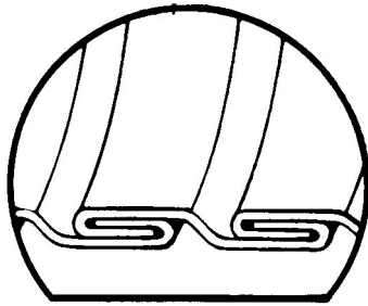
Cut-away-photo view and detail drawing of construction
